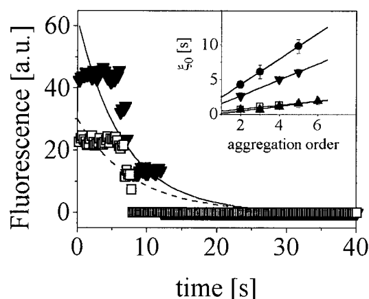
FIGURE 5 Typical fluorescence kinetics for aggregates of rhodamine 6G molecules: a fourth order aggregate (▼) and a second order aggregate (□). Solid and dashed lines are the best fit to an exponential decay for the fourth and the second order aggregate kinetics, respectively. Inset: average decay time obtained by fitting the aggregate kinetics to a single exponential decay, \xi_N , versus the order of aggregation for Fluorescein (▼), Rhodamine 6G (●), Pyrene (▲), and Indo-1 (□). The solid lines are the linear fits, \xi_N = N \xi_0 . The values of \xi_0 for the four dyes are reported in Table 1.
